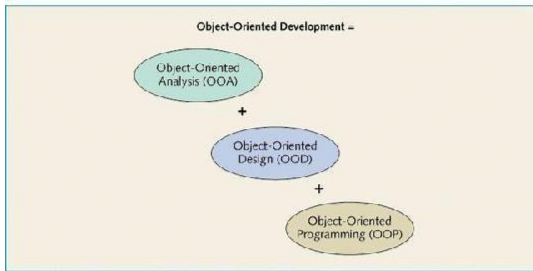
Figure 1-3 Object-oriented development
