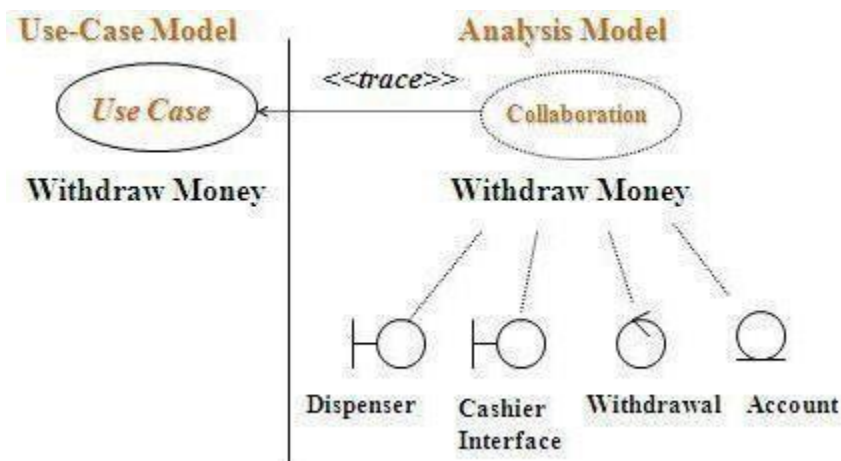
A collaboration diagram for the Withdraw Money use-case realization in the analysis model
