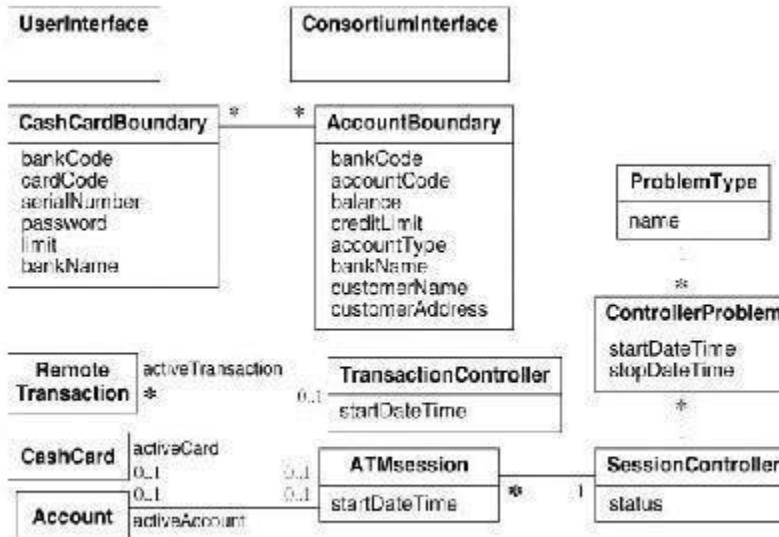
Figure 13.8 ATM application class model. Application classes augment the domain classes and are necessary for developers.
