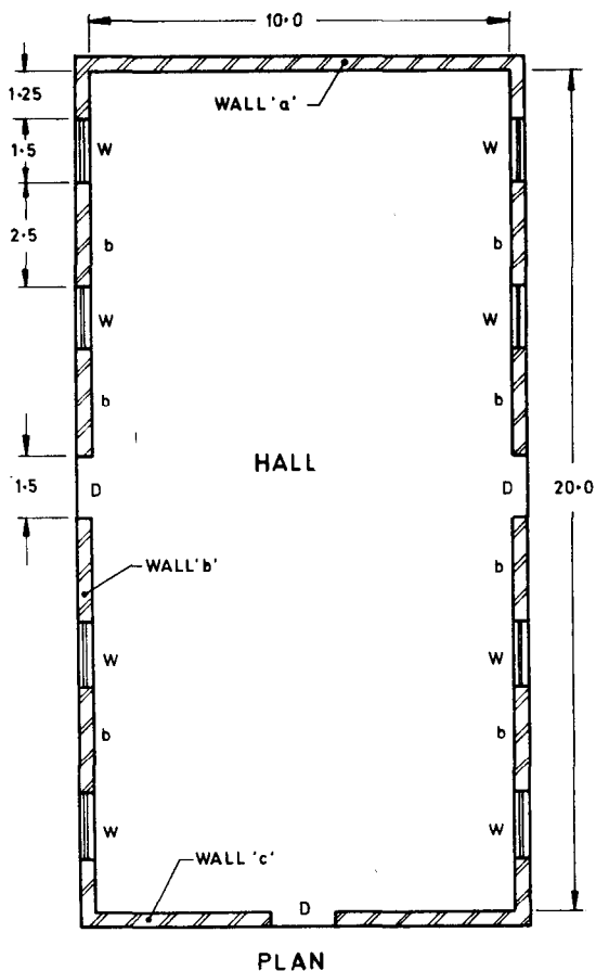
PLAN All dimensions in metres.
