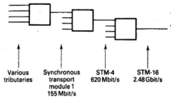
Figure 1.25 the SDH
