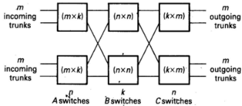
Figure 4.9.Space division equivalent of S-T-S switch: m= number of PCM highways, n=number of Time slots, k= number of time switch links.
