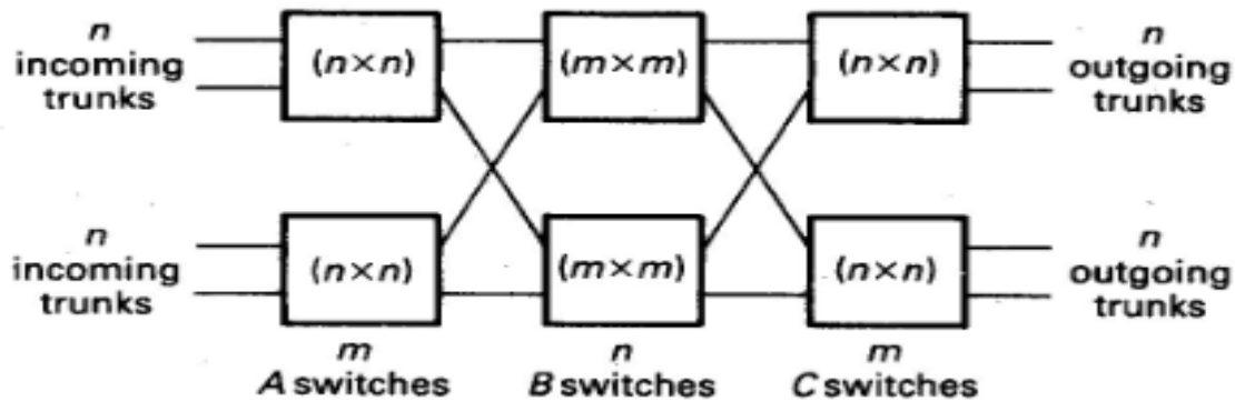
Figure 4.10 Space division equivalent of T-S-T switch. M = number of PCM highways n = number of time slots.
