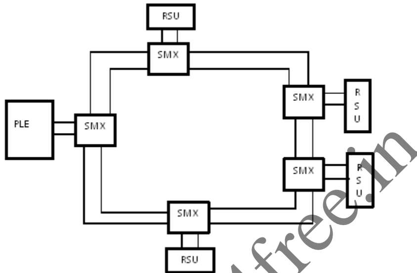
Fig 1.27 Local exchanges connected by synchronous ring. SMX= synchronous mux. PLE=Principal local exchange. RSU=Remote switching unit.
