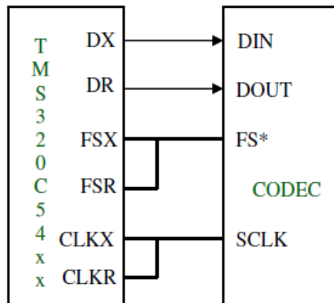
Fig. 8.1: SSI between DSP & CODEC
