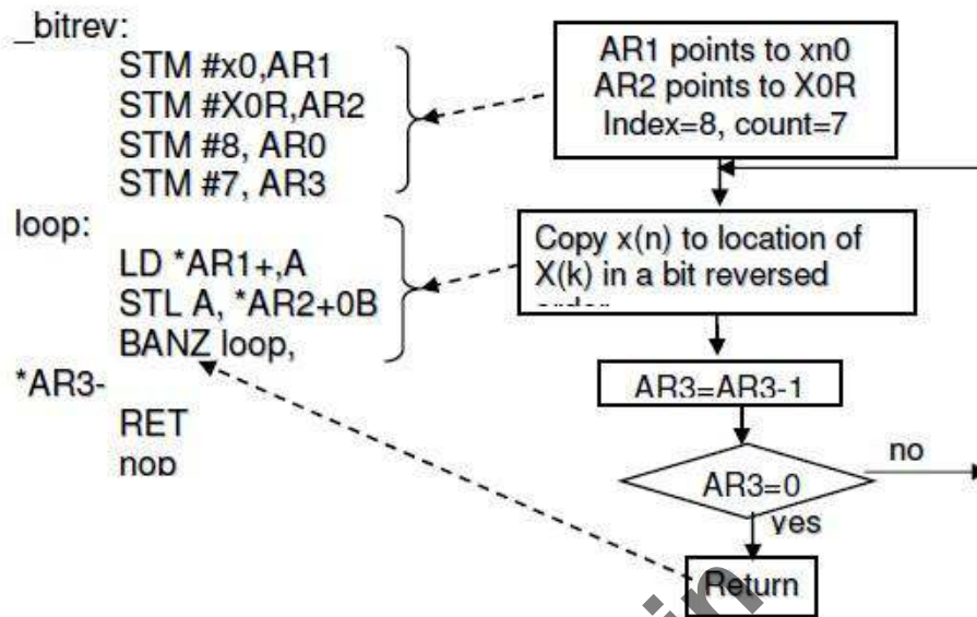
Fig. 6.12: Bit Reverse Subroutine
