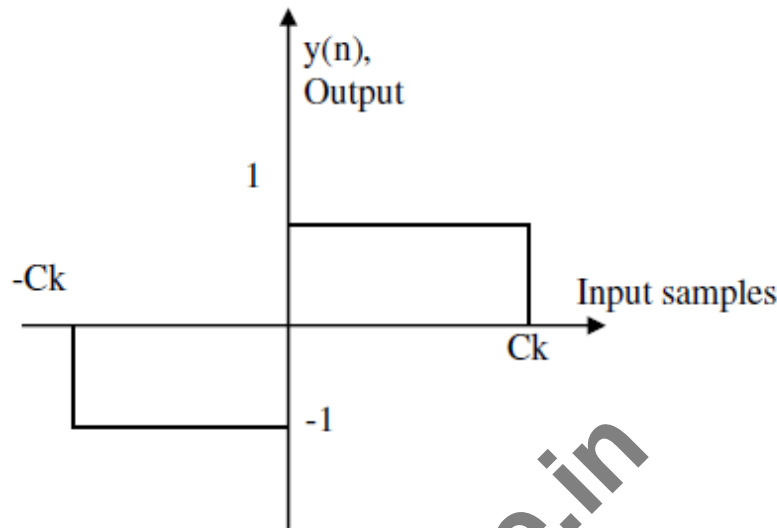
Fig. 8.18: Center Clipper
