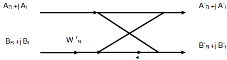
Fig 6. 3: Butterfly structure for N point DITFFT Computation
