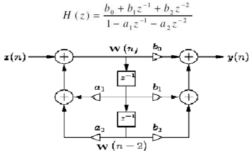
Figure 5.4 Block diagram of second order IIR filter
