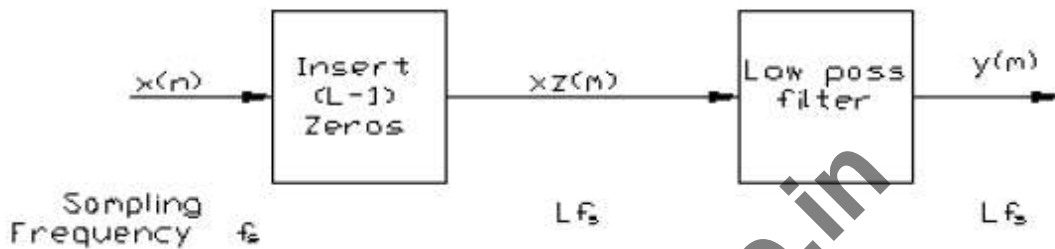
Fig 1.13 Interpolation Process
