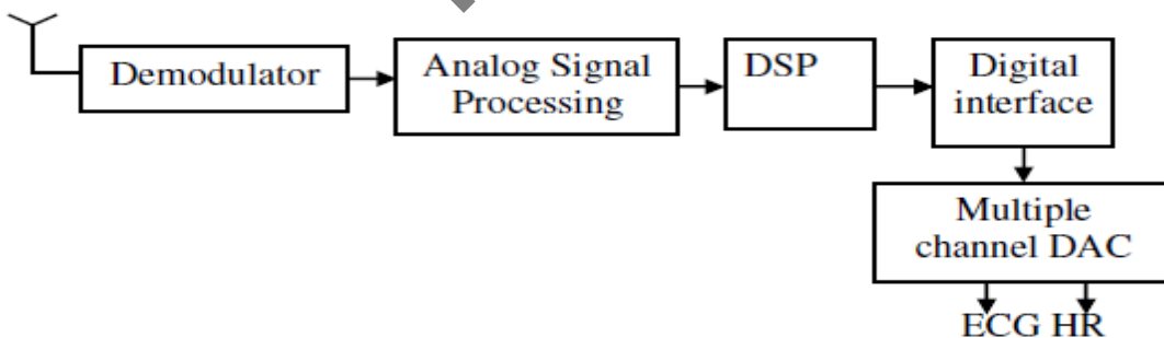
Fig. 8.8: Bio-telemetry Receiver
