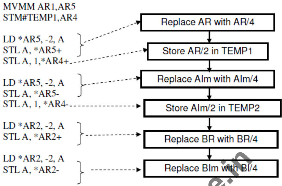
Fig. 6.13: Butterfly Subroutine
