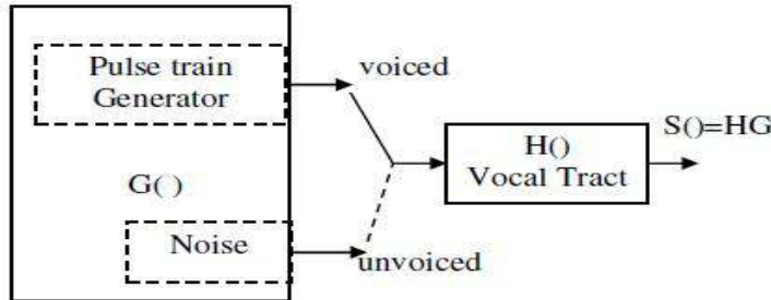
Fig. 8.14: Speech Production Model
