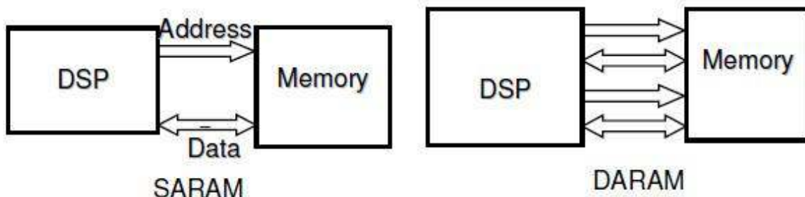
Fig. 7.3: SARAM & DARAM
