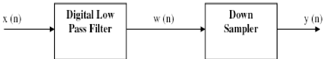
Fig 1.12 Decimation Process
