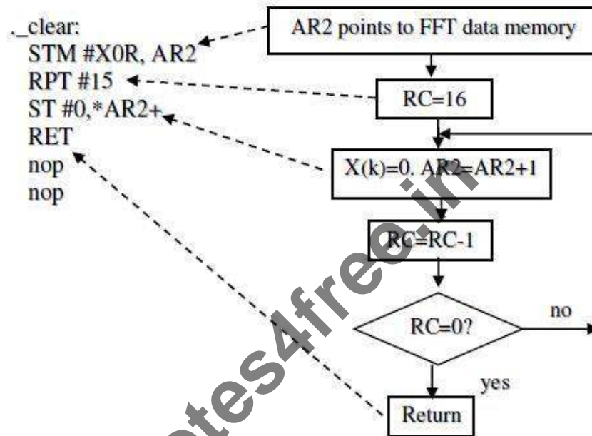
Fig. 6.11: Clear subroutine
