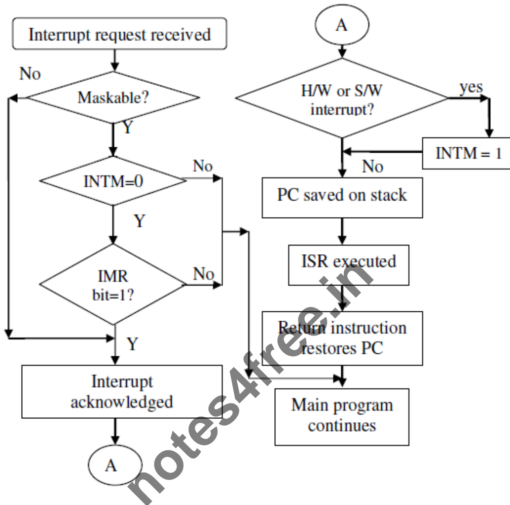
Fig. 7.9: Response of DSP to interrupt
