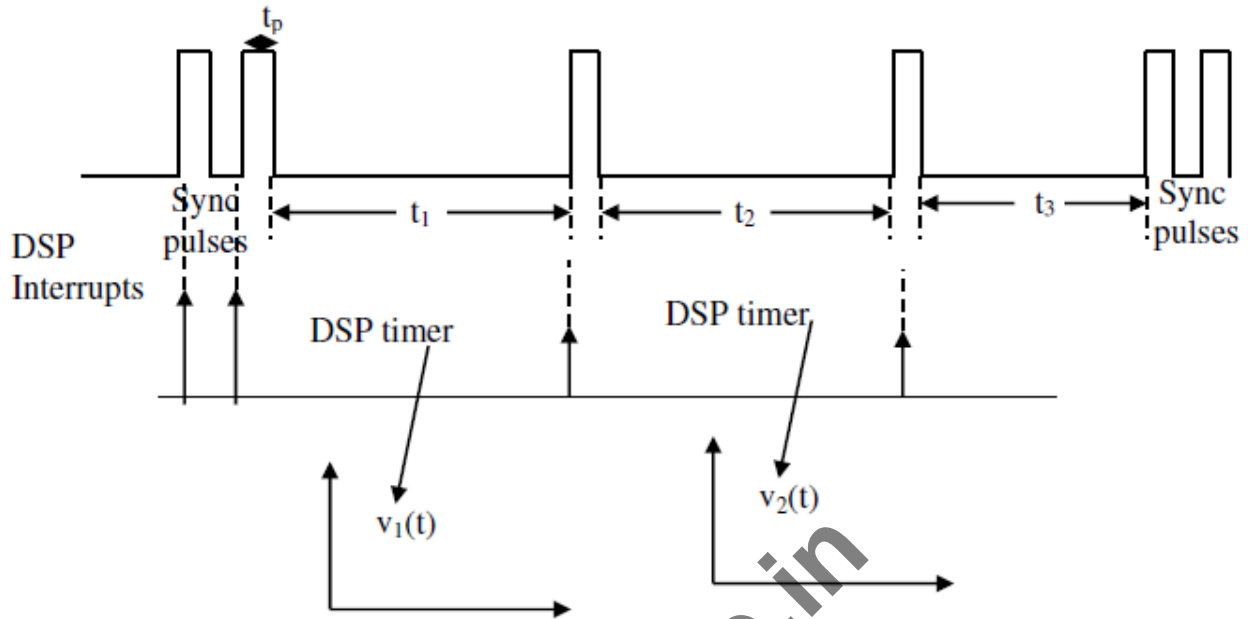
Fig. 8.10: Decoding PPM signal with two ECG signals
