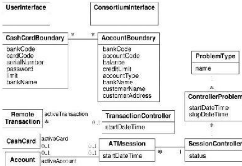
Figure 13.8. ATM application class model. Application classes augment the domain classes and are necessary for development.
