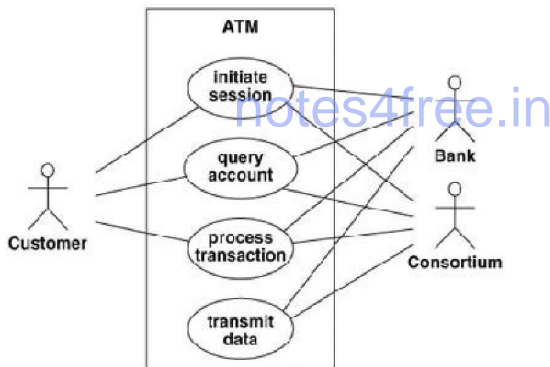
Figure 13.1 Use case diagram for the ATM. Use cases partition the
